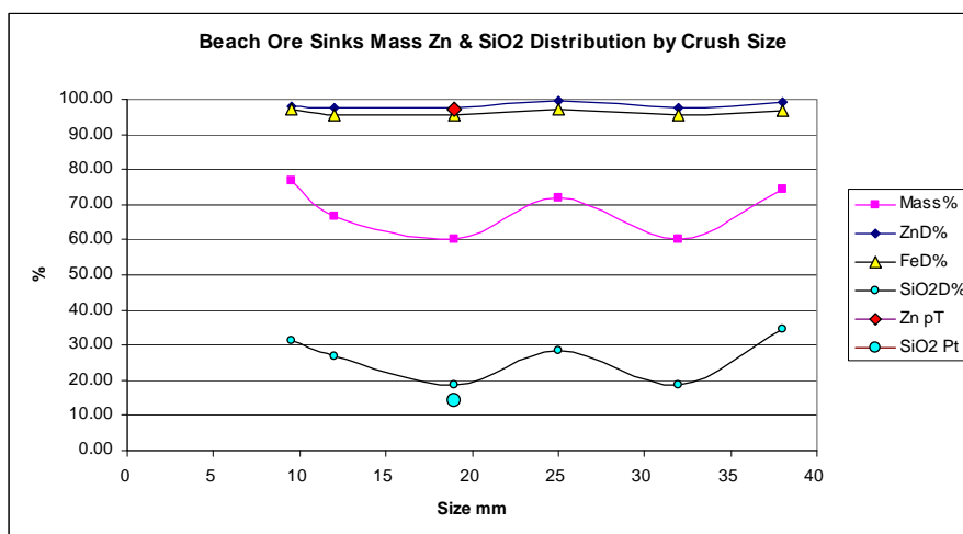
Figure 6 DMS size results for Beach L2
