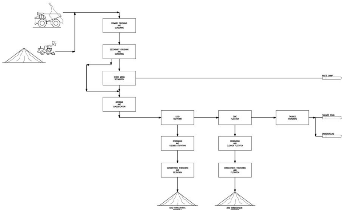
Figure 10 Overall process flowsheet
