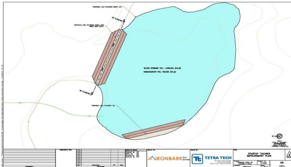
Figure 14 Lake Platinova dam
